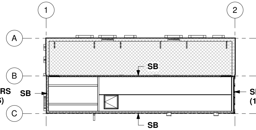
2 SANDBLASTING PLAN - 2ND CONTAINER LEVEL 1:150
